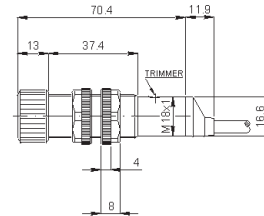
M12 CONNECTOR
