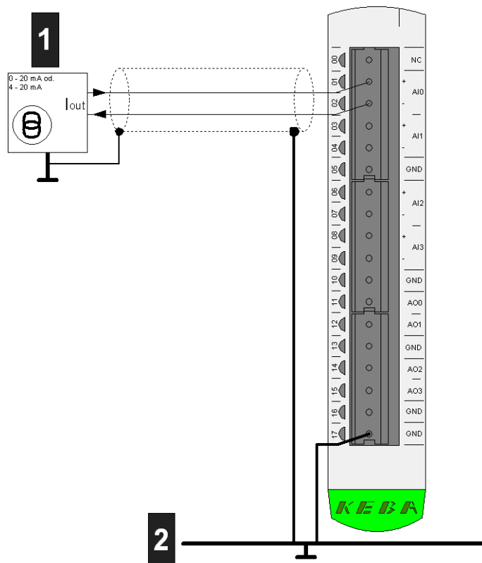
Fig.4-2: Connection example for analog inputs
