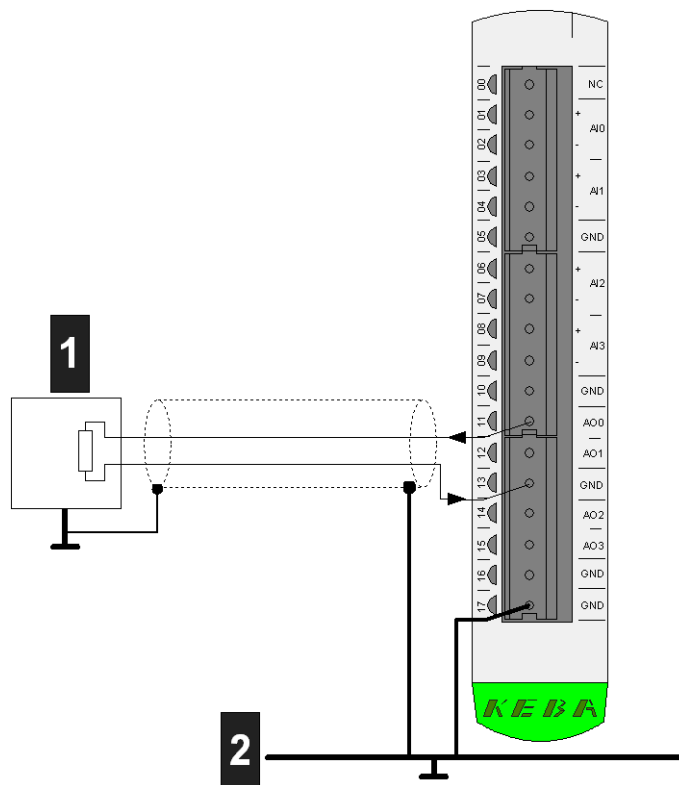
Fig.4-4: Connection example for analog outputs
