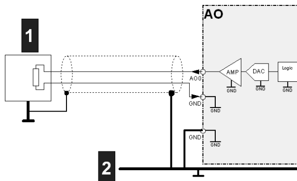
Fig.4-5: Connection diagram for analog outputs
