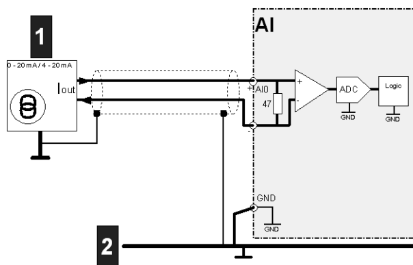
Fig.4-3: Connection diagram analog inputs
