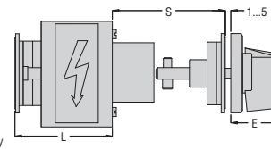
4-screw drilling for GN125 handle and "4V" suffix types only
