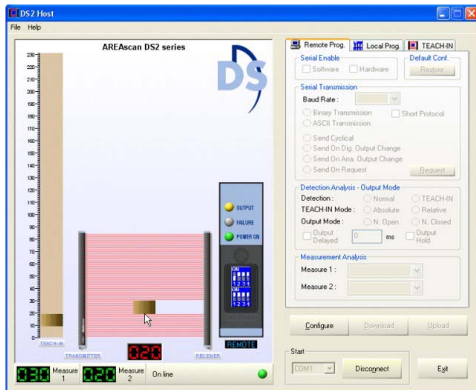
Fig. 15 - DS2 Graphic user interface
