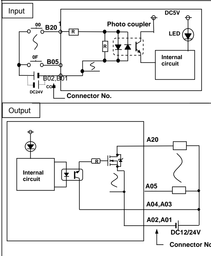
Circuit configuration
